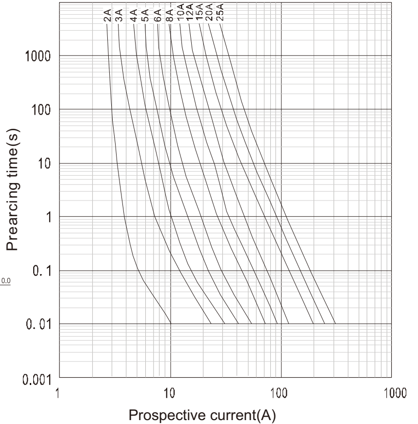
AVERAGE I-T CHARACTERISTICS CURVE (FOR REFERENCE ONLY)
