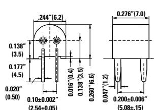
Circuit Board Mounting Detail
