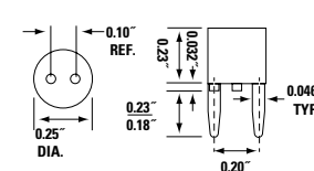
Circuit Board Mounting Detail
